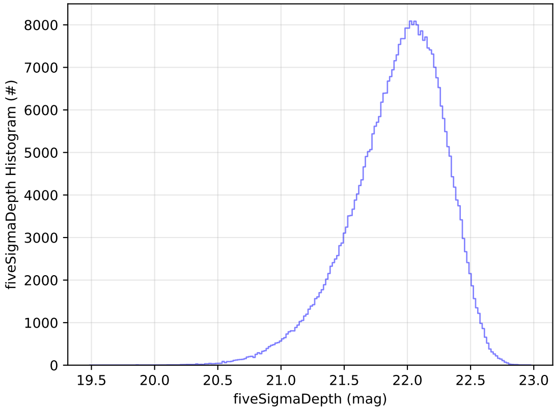
weather_cloudso16v3.5_10yrs y: fiveSigmaDepth Histogram
