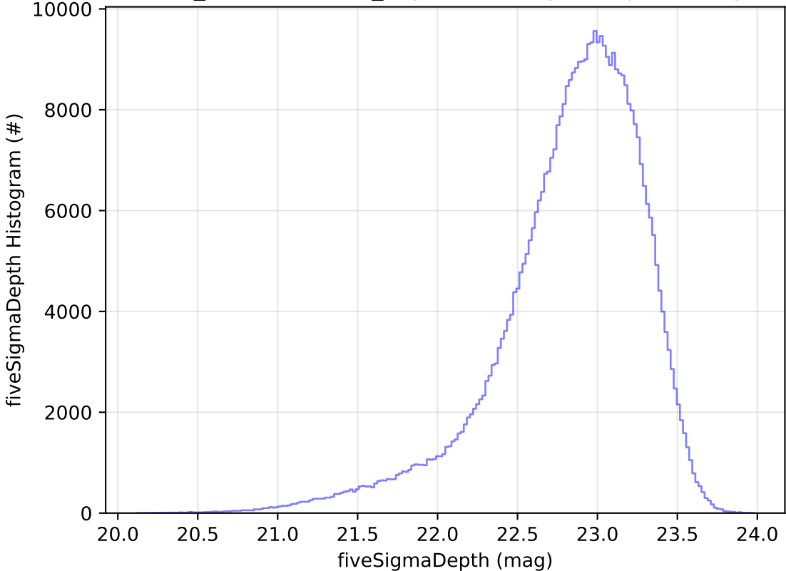
weather_cloudso16v3.5_10yrs z: fiveSigmaDepth Histogram
