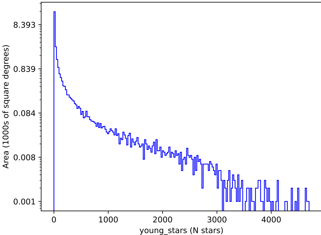
weather_cloudso16v3.5_10yrs : young_stars
