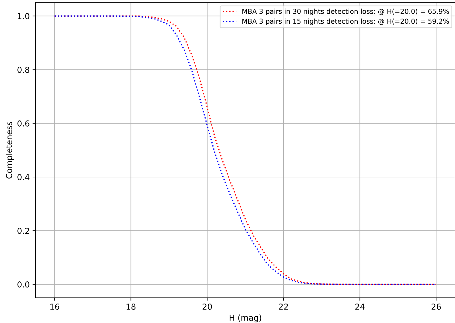
weather_cloudso16v3.5_10yrs: DifferentialCompleteness
