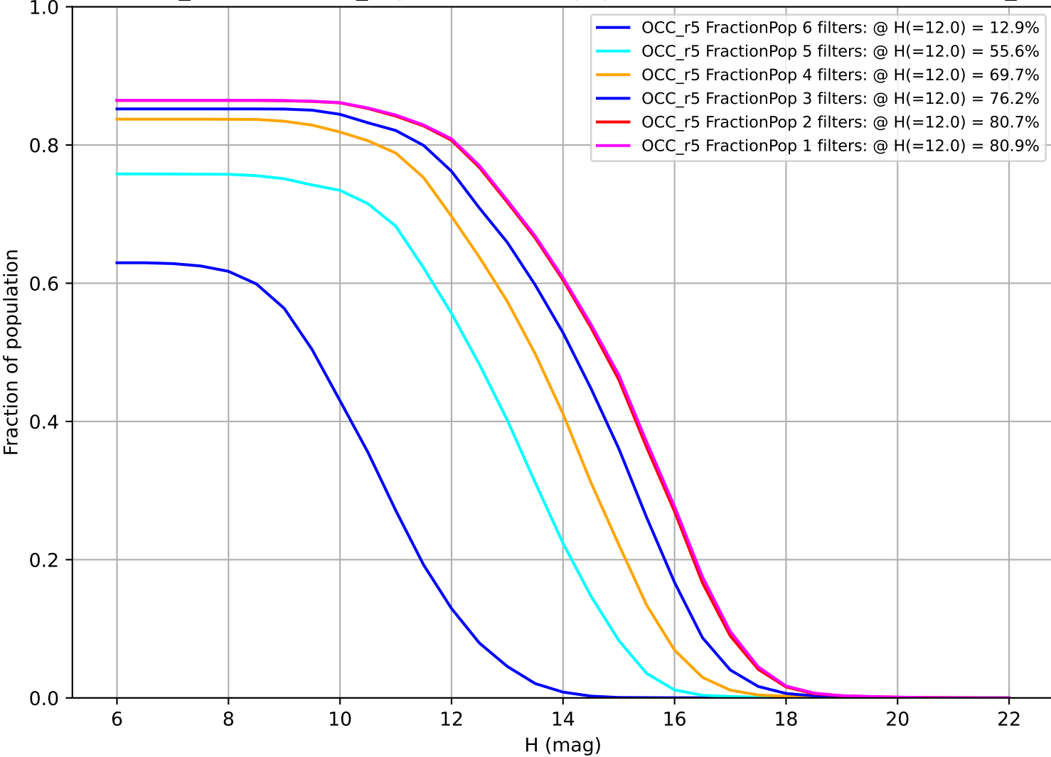
weather_cloudso16v3.5_10yrs: Fraction of population with colors in X filters OCC_r5
