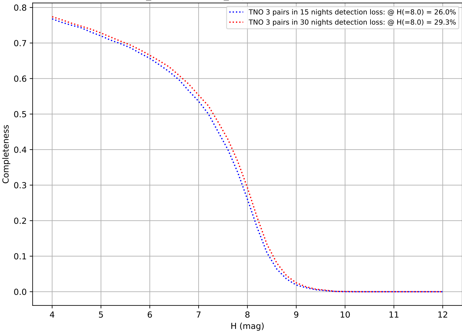
weather_cloudso16v3.5_10yrs: DifferentialCompleteness
