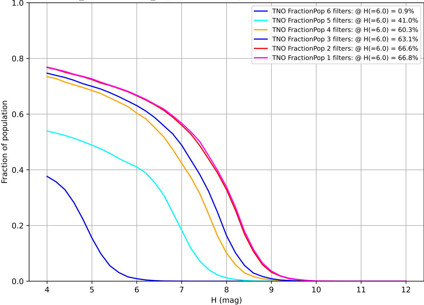
weather_cloudso16v3.5_10yrs: Fraction of population with colors in X filters TNO
