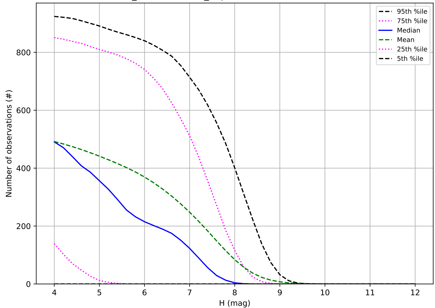
weather_cloudso16v3.5_10yrs: Number of observations TNO
