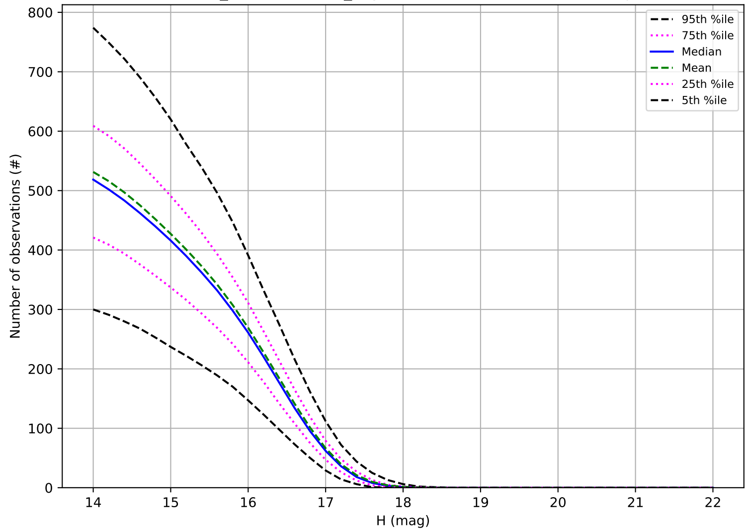
weather_cloudso16v3.5_10yrs: Number of observations Trojan
