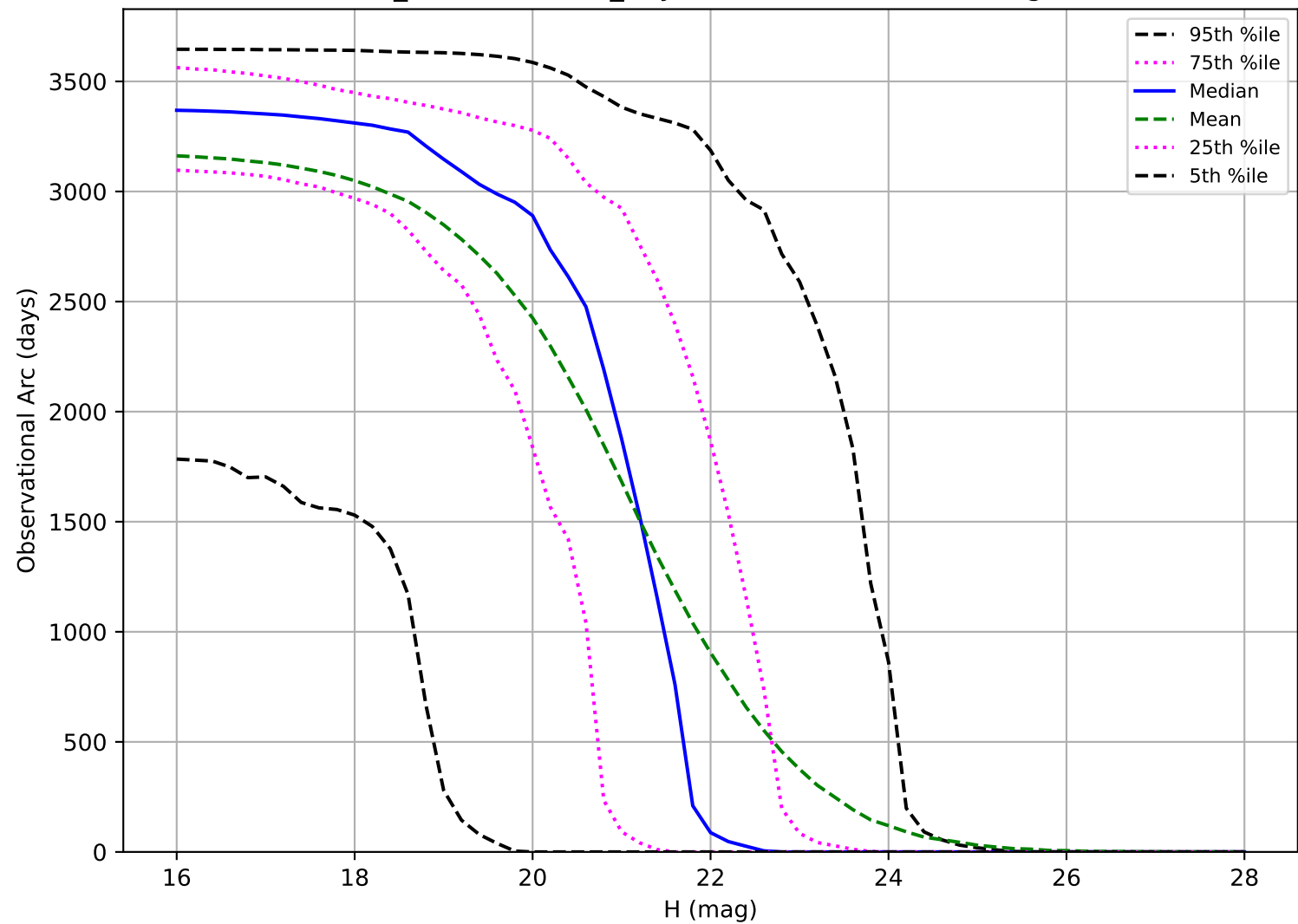
weather_cloudso16v3.5_10yrs: Observational Arc Length NEO
