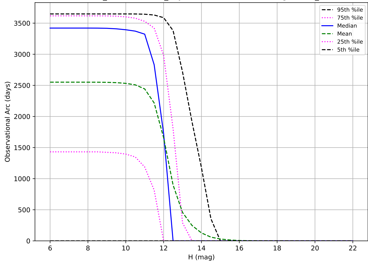
weather_cloudso16v3.5_10yrs: Observational Arc Length OCC_r20
