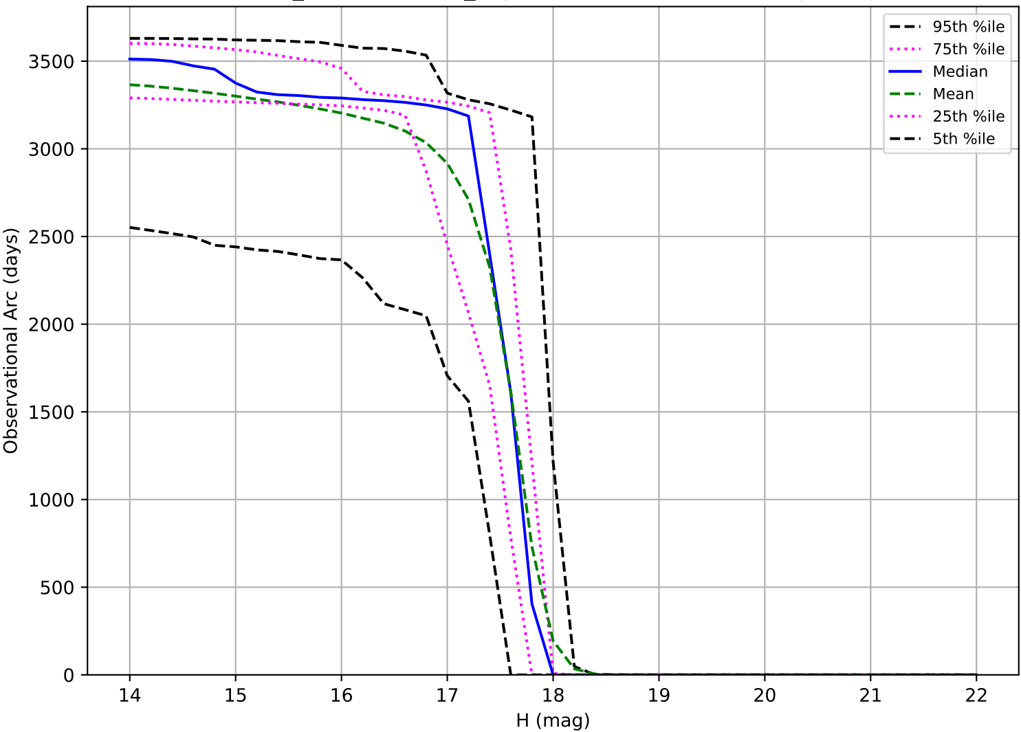
weather_cloudso16v3.5_10yrs: Observational Arc Length Trojan
