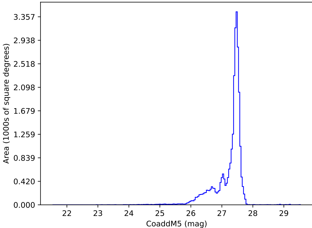
weather_cloudso18v3.5_10yrs : CoaddM5
