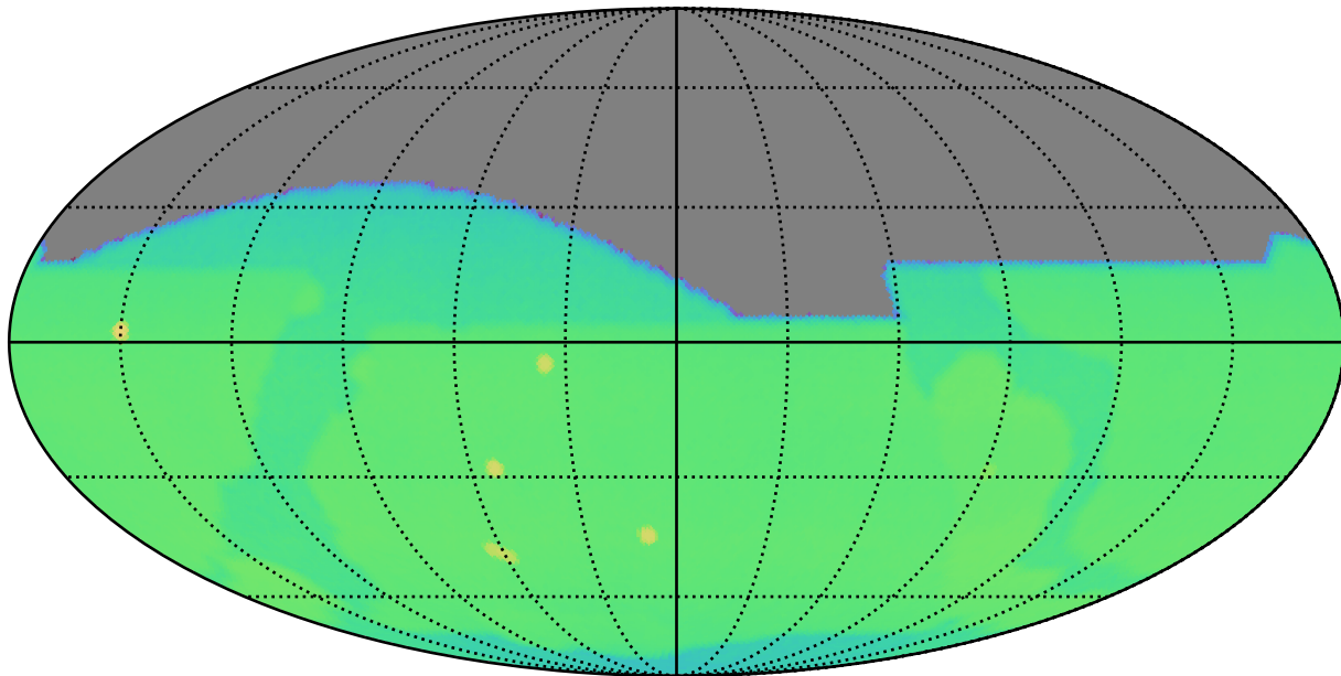
weather_cloudso18v3.5_10yrs : CoaddM5
