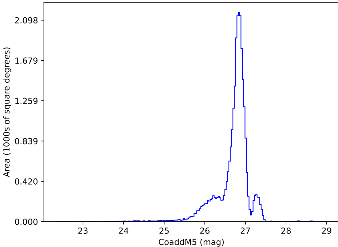
weather_cloudso18v3.5_10yrs g: CoaddM5
