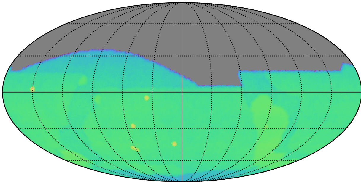
weather_cloudso18v3.5_10yrs g: CoaddM5
