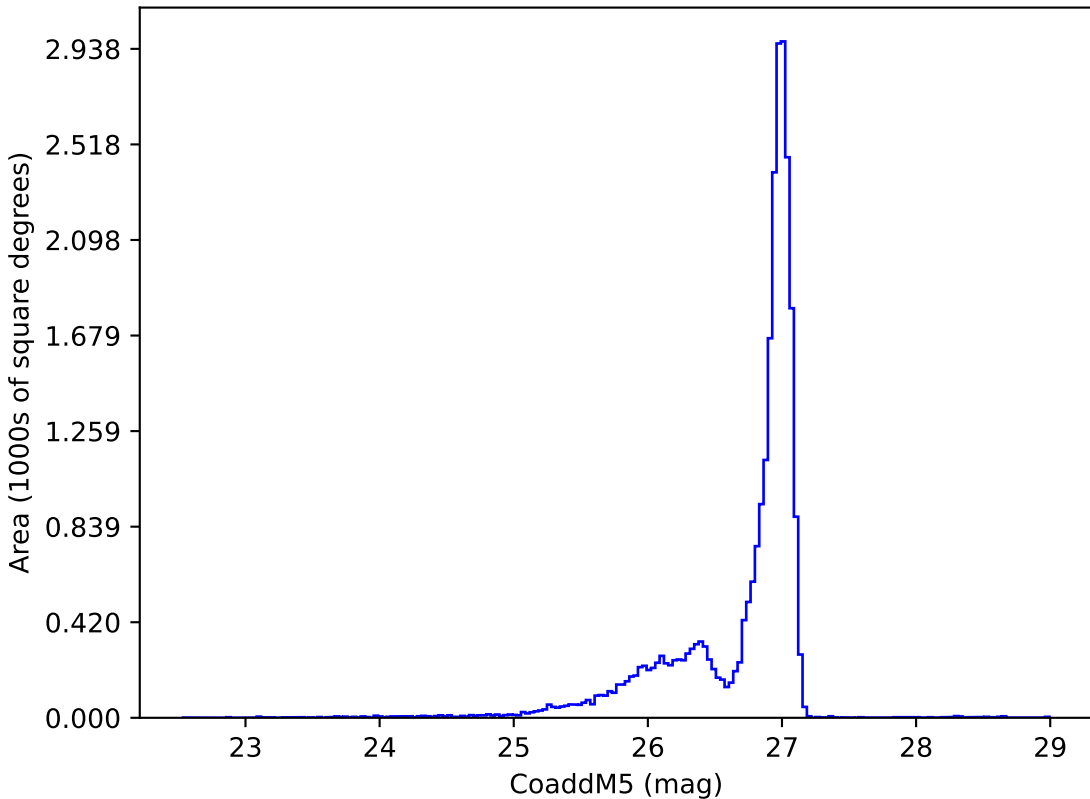
weather_cloudso18v3.5_10yrs r: CoaddM5
