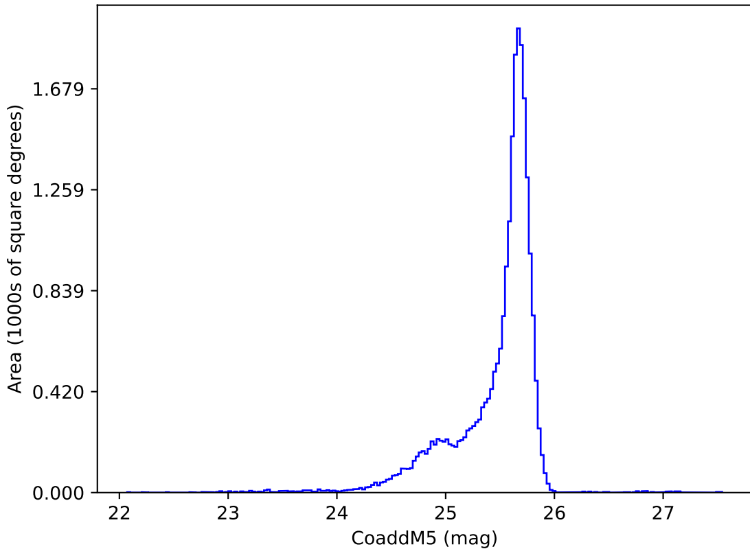
weather_cloudso18v3.5_10yrs u: CoaddM5
