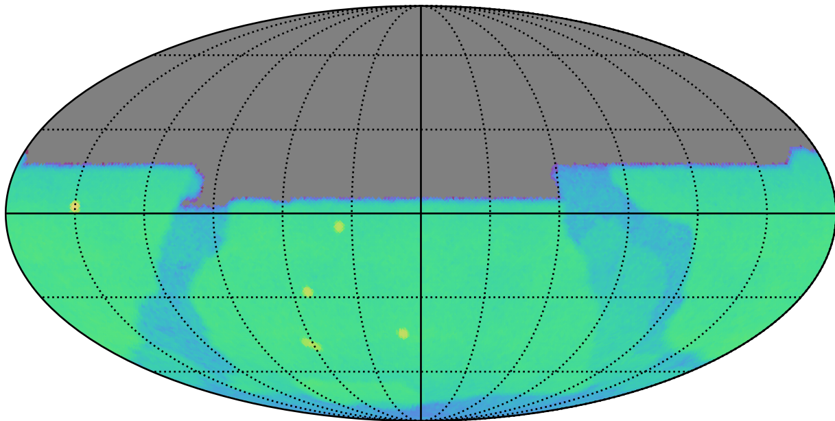
weather_cloudso18v3.5_10yrs u: CoaddM5
