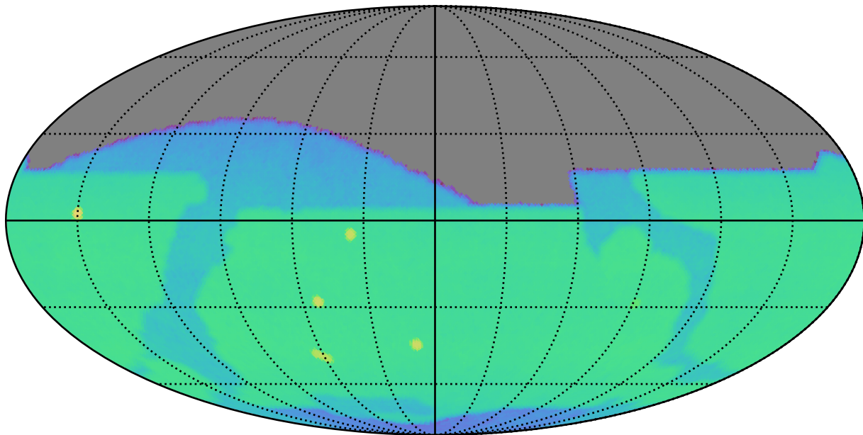
weather_cloudso18v3.5_10yrs z: CoaddM5
