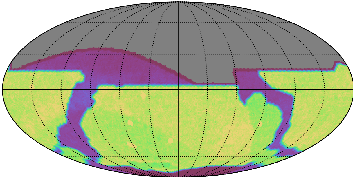
weather_cloudso18v3.5_10yrs : Count observationStartMJD
