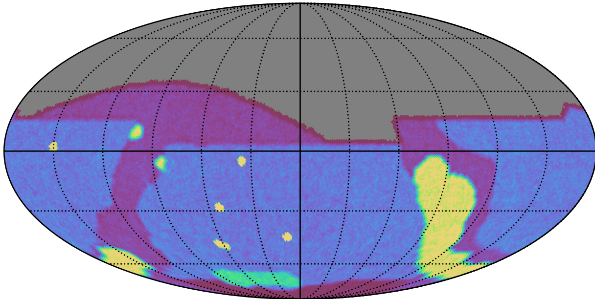
weather_cloudso18v3.5_10yrs g: Count observationStartMJD
