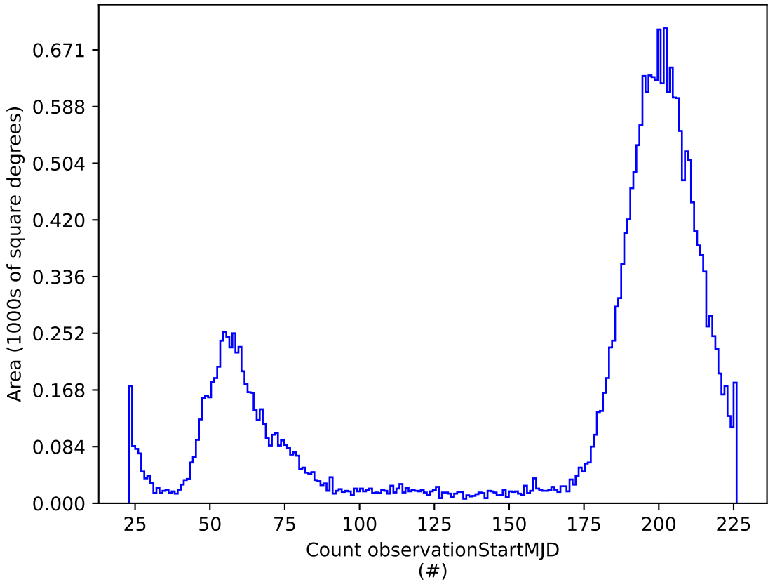
weather_cloudso18v3.5_10yrs i: Count observationStartMJD
