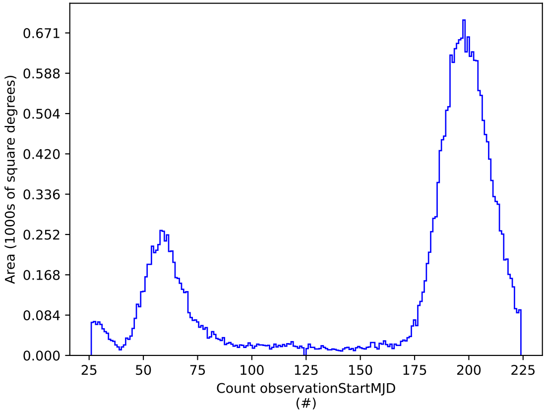
weather_cloudso18v3.5_10yrs r: Count observationStartMJD
