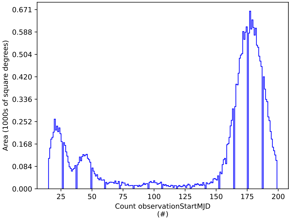
weather_cloudso18v3.5_10yrs y: Count observationStartMJD
