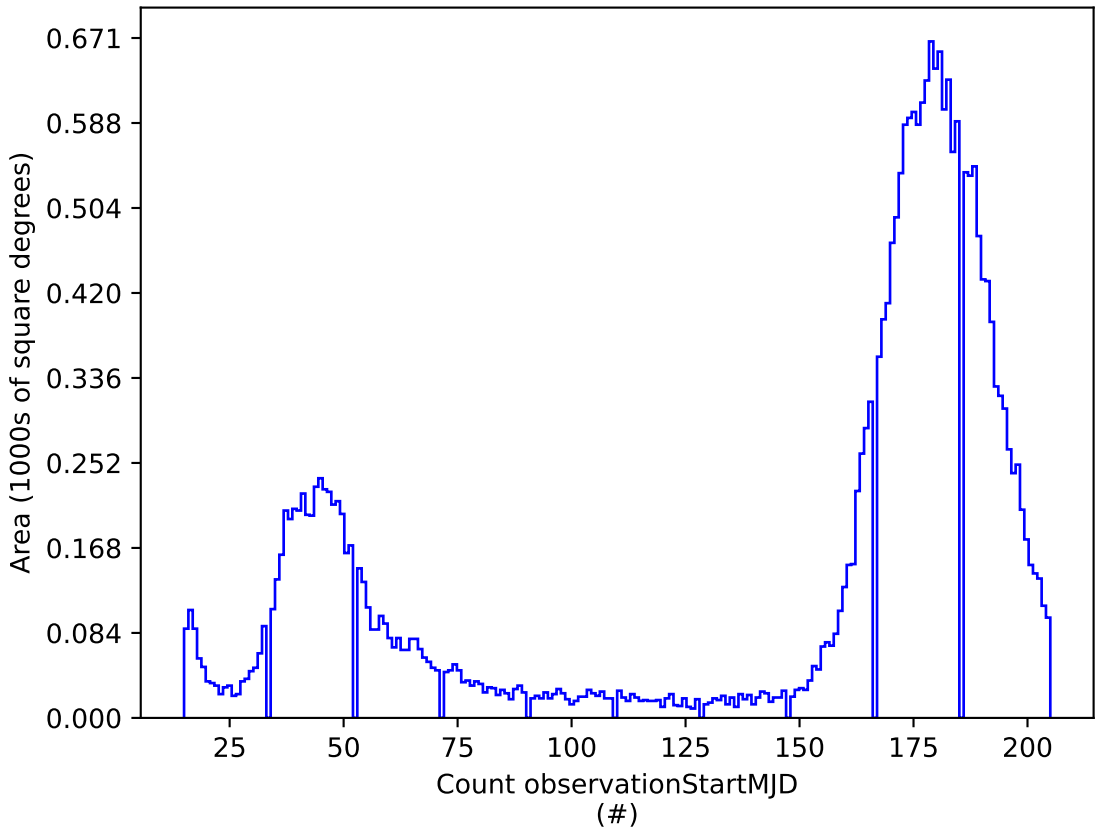
weather_cloudso18v3.5_10yrs z: Count observationStartMJD
