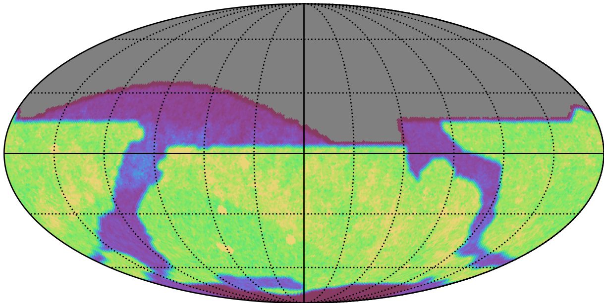
weather_cloudso18v3.5_10yrs z: Count observationStartMJD
