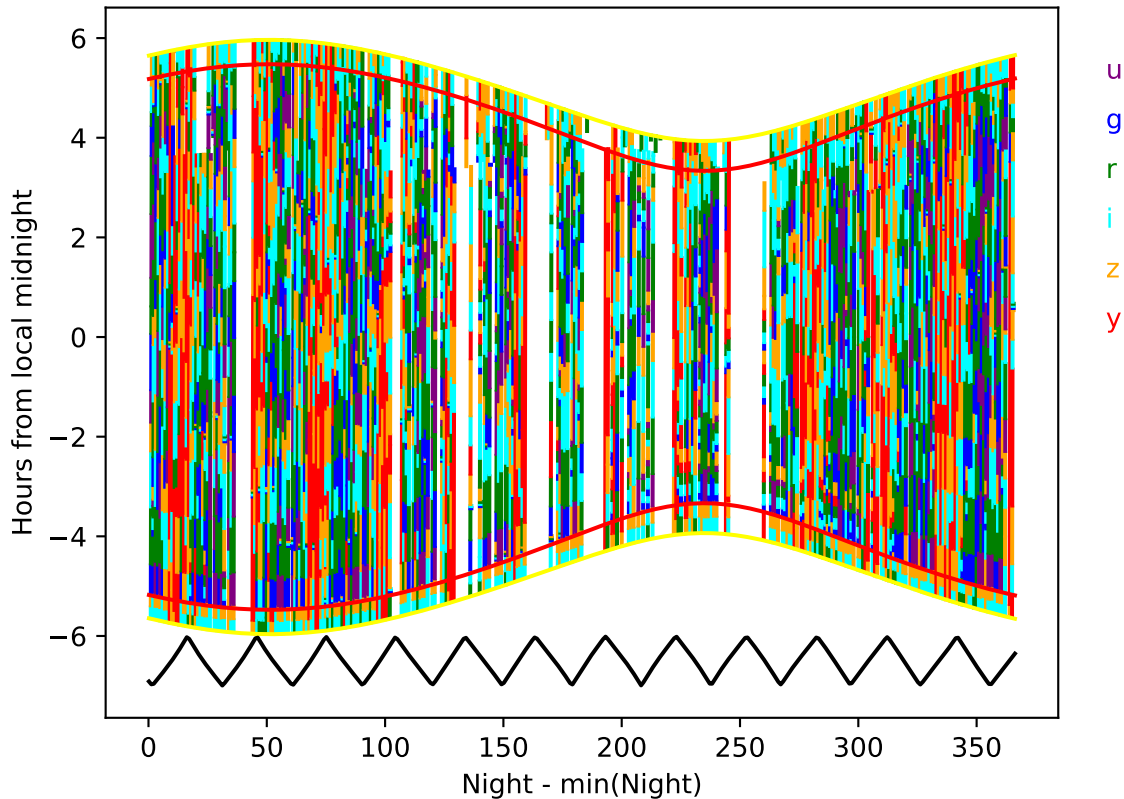
weather_cloudso18v3.5_10yrs year 5-6: Hourglass
