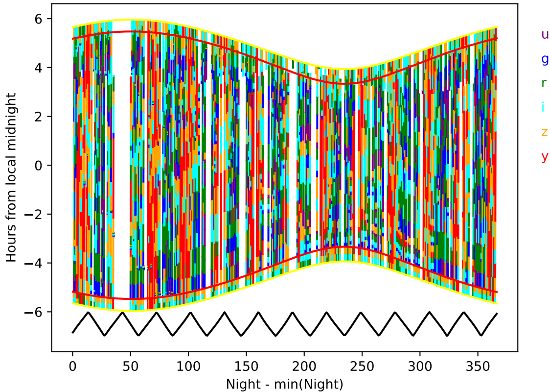
weather_cloudso18v3.5_10yrs year 8-9: Hourglass
