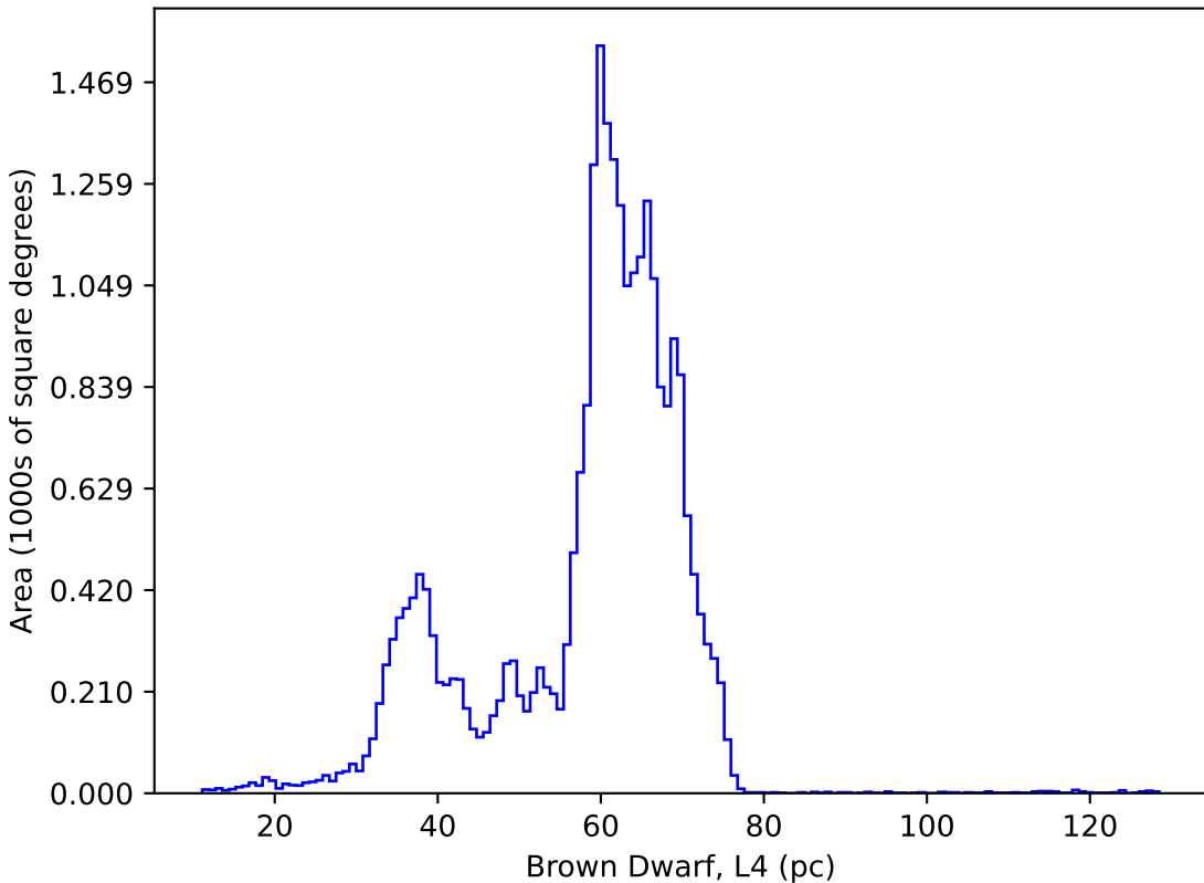
weather_cloudso18v3.5_10yrs : Brown Dwarf, L4
