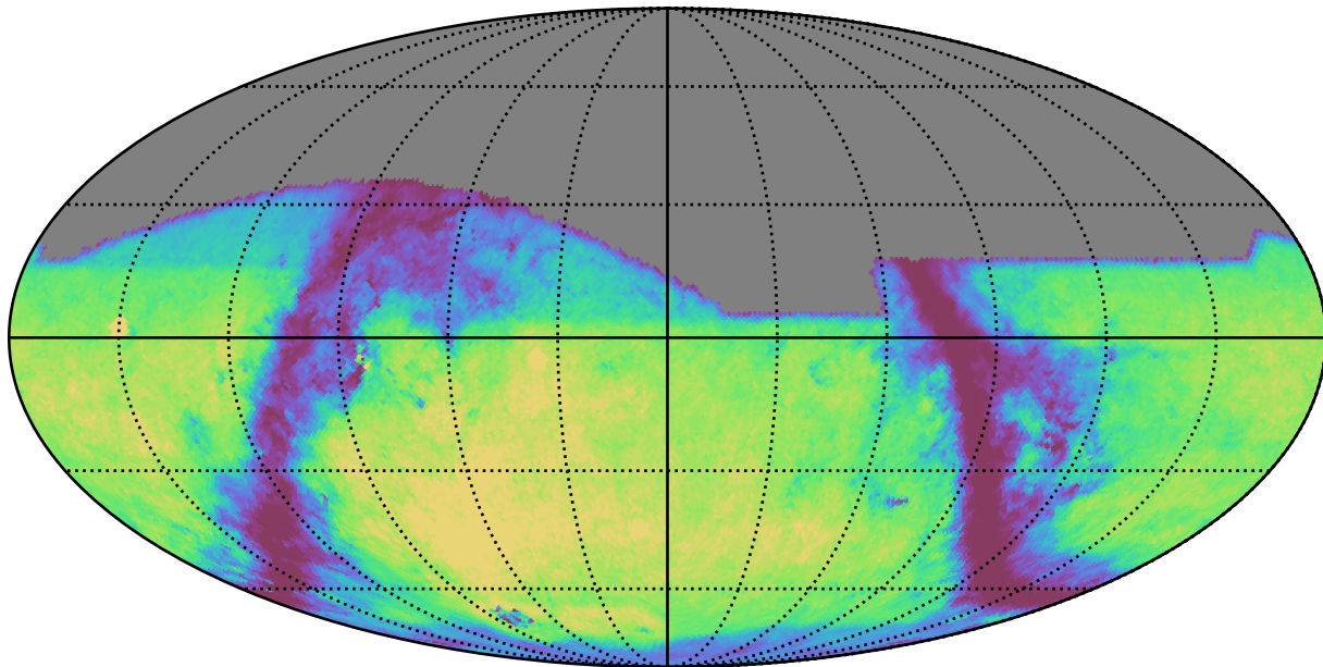
weather_cloudso18v3.5_10yrs g: GalaxyCountsMetricExtended
