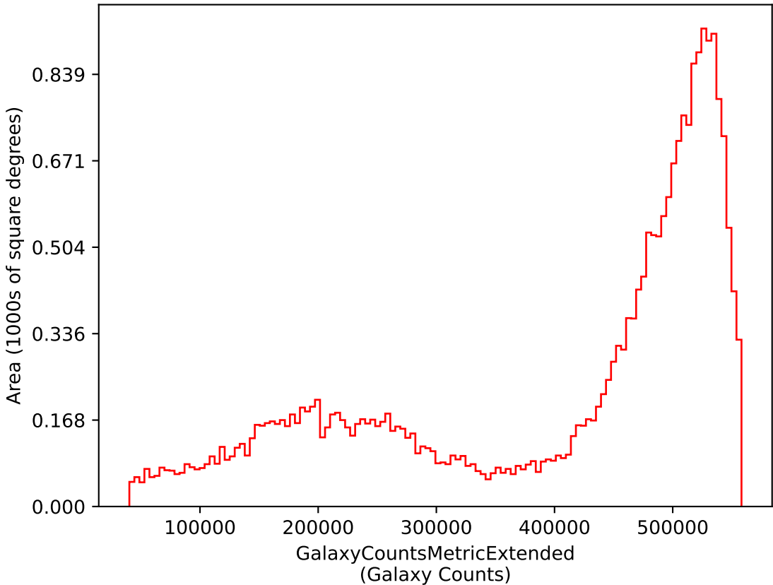
weather_cloudso18v3.5_10yrs i: GalaxyCountsMetricExtended
