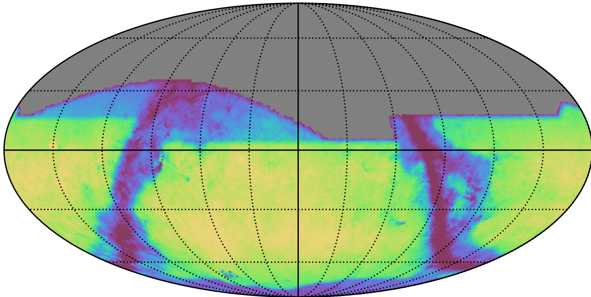
weather_cloudso18v3.5_10yrs i: GalaxyCountsMetricExtended
