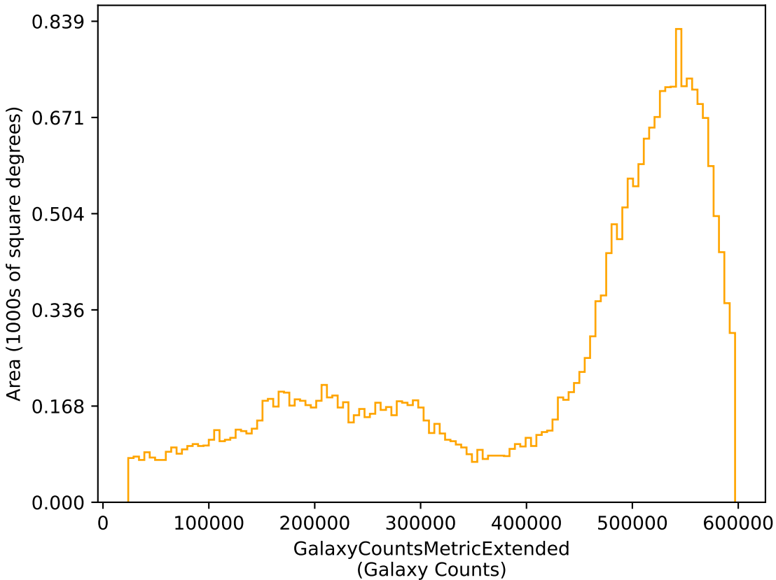
weather_cloudso18v3.5_10yrs r: GalaxyCountsMetricExtended
