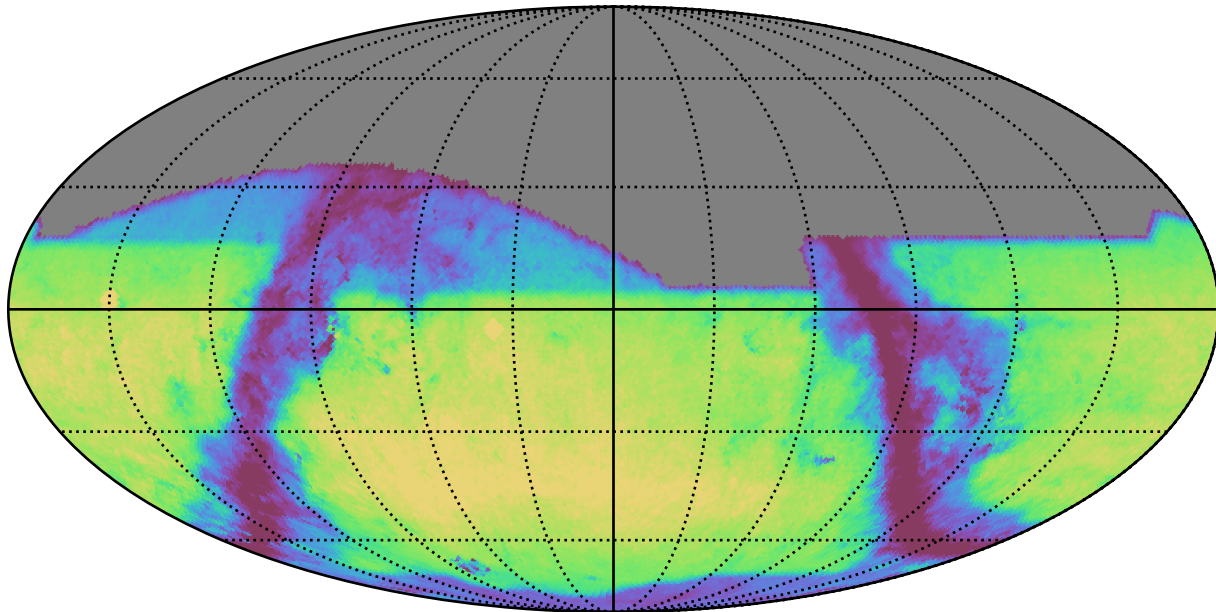
weather_cloudso18v3.5_10yrs r: GalaxyCountsMetricExtended
