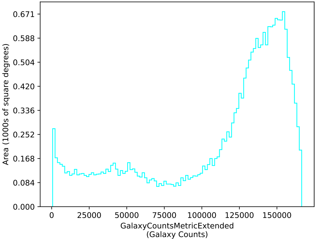
weather_cloudso18v3.5_10yrs u: GalaxyCountsMetricExtended
