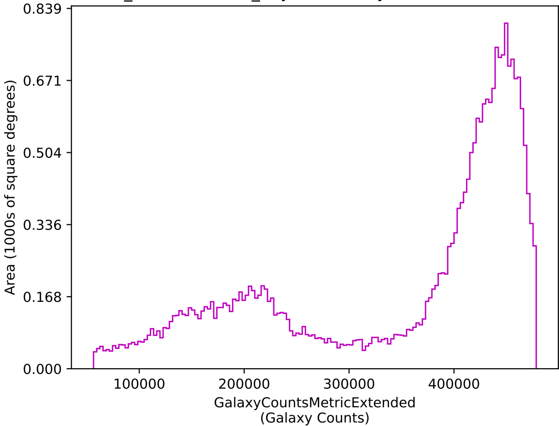
weather_cloudso18v3.5_10yrs z: GalaxyCountsMetricExtended
