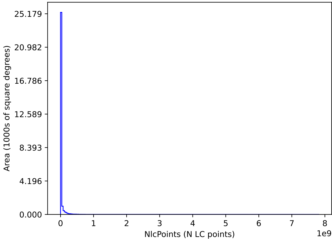
weather_cloudso18v3.5_10yrs : NlcPoints
