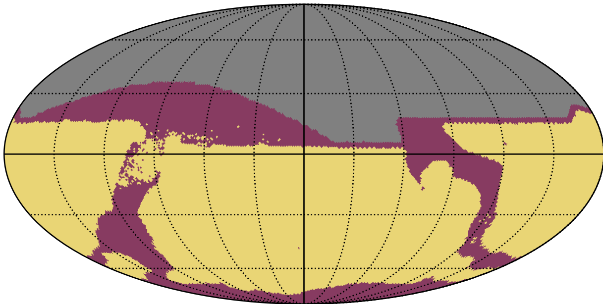
weather_cloudso18v3.5_10yrs : RapidRevisits
