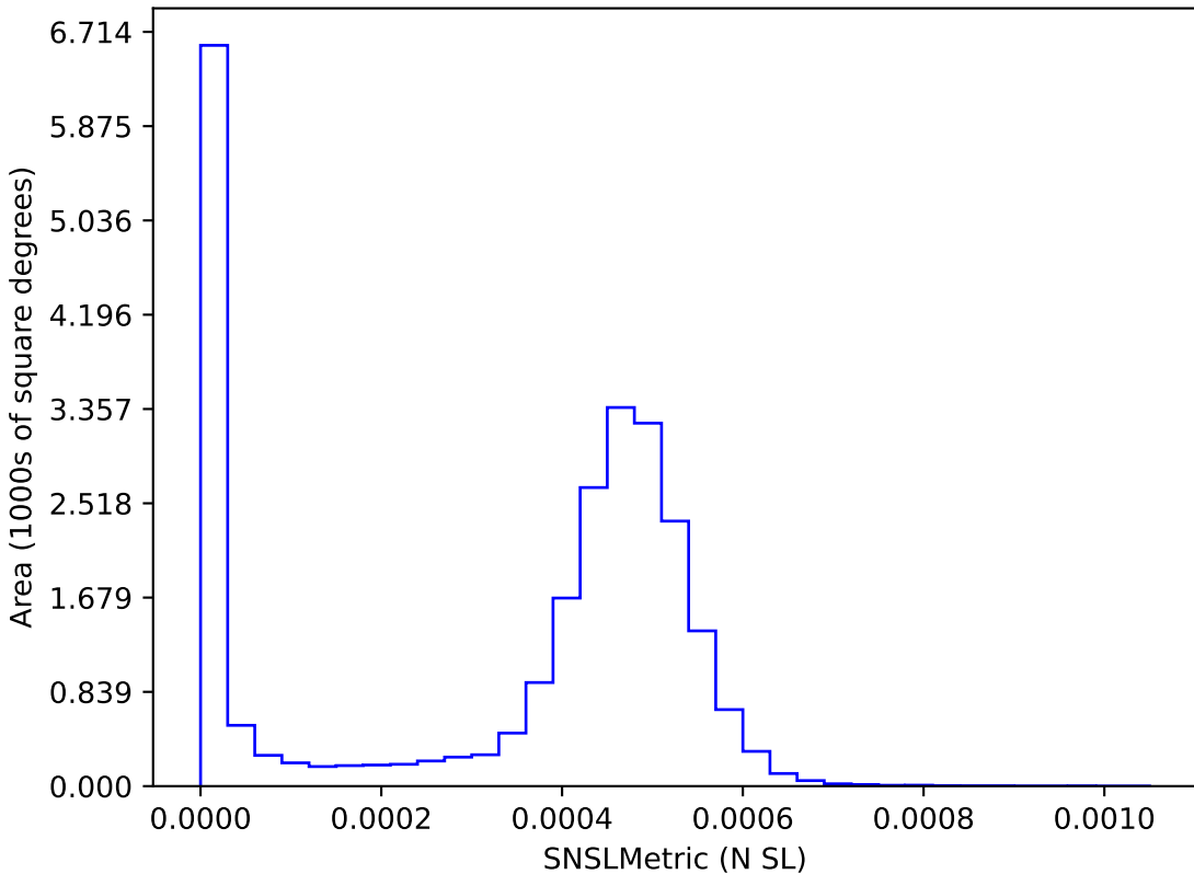
weather_cloudso18v3.5_10yrs : SNSLMetric
