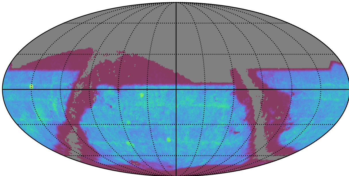
weather_cloudso18v3.5_10yrs : SNSLMetric
