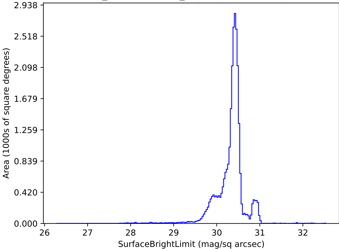
weather_cloudso18v3.5_10yrs g: SurfaceBrightLimit
