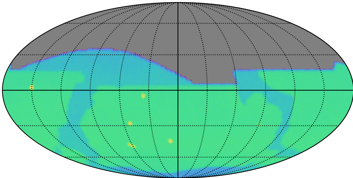
weather_cloudso18v3.5_10yrs r: SurfaceBrightLimit
