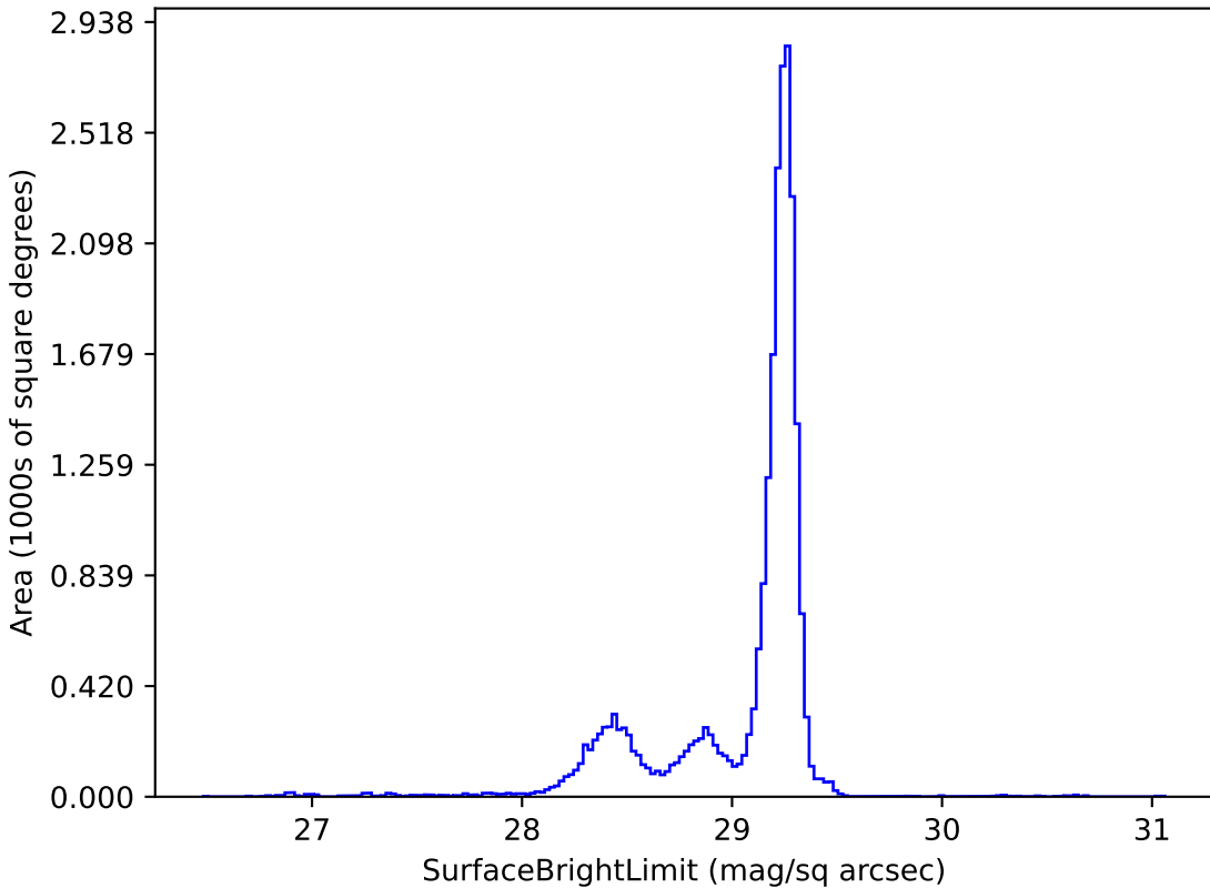
weather_cloudso18v3.5_10yrs u: SurfaceBrightLimit
