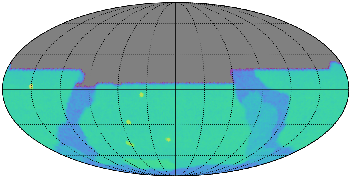
weather_cloudso18v3.5_10yrs u: SurfaceBrightLimit
