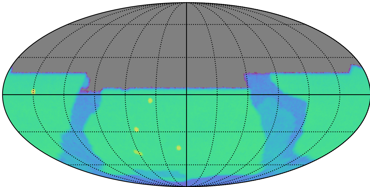
weather_cloudso18v3.5_10yrs y: SurfaceBrightLimit
