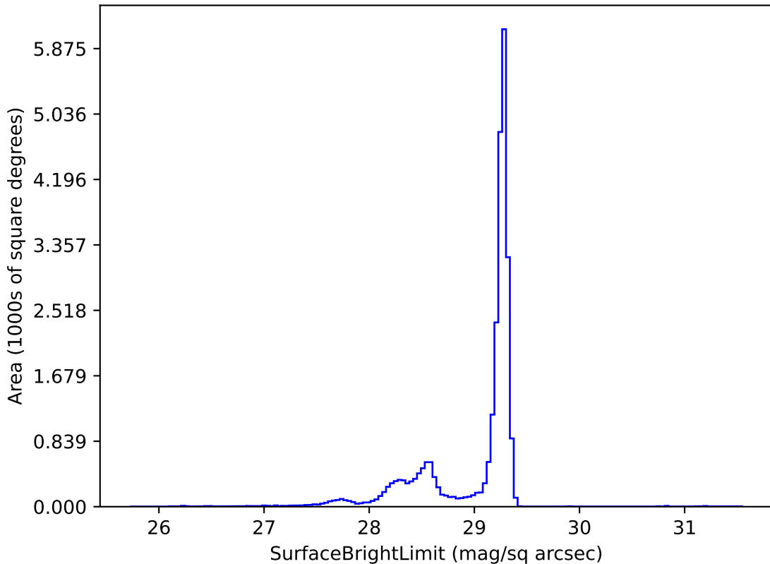
weather_cloudso18v3.5_10yrs z: SurfaceBrightLimit
