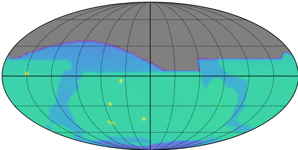
weather_cloudso18v3.5_10yrs z: SurfaceBrightLimit
