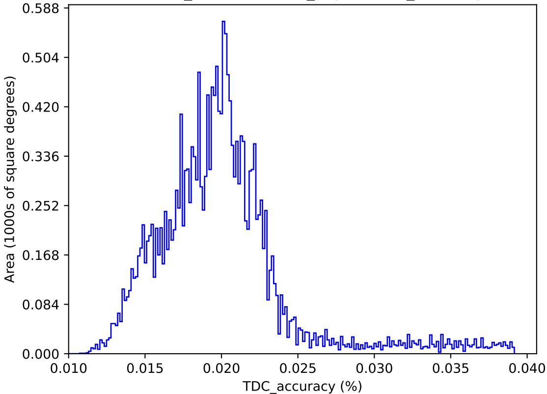
weather_cloudso18v3.5_10yrs : TDC_accuracy
