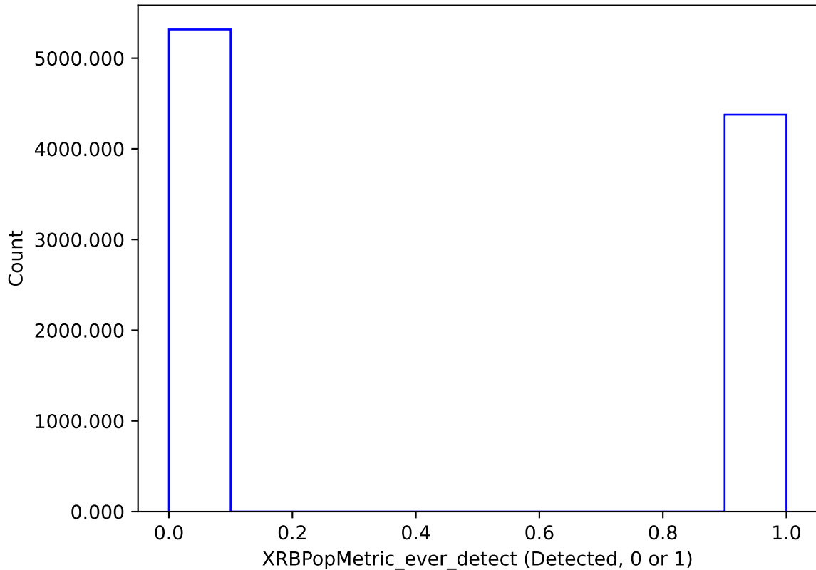
weather_cloudso18v3.5_10yrs : XRBPoMetric_ever_detect
